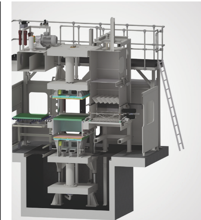
FULLY AUTOMATIC PRESSING SYSTEM WPA 1000 S FOR PRODUCTION OF VIP PANELS
